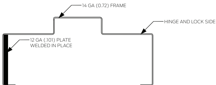
Detail 2, Level 2 and 3, Armor Reinforcement
